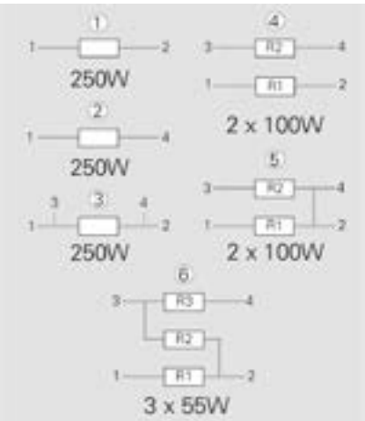
Version 5: ohmic value between contact 2 and 4 aprox. 3mΩ
