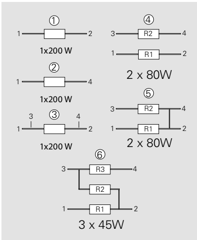
Version 5: ohmic value between contact 2 and 4 aprox. 3mΩ
